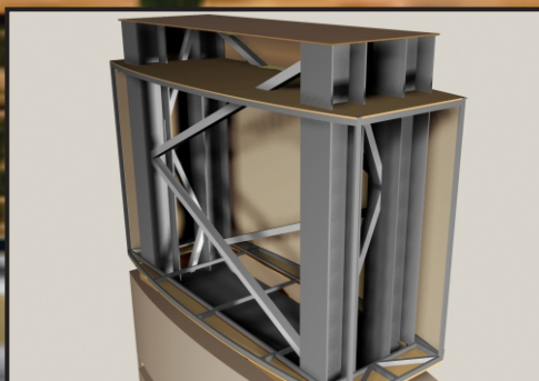
Structural & Base Steel Installation
